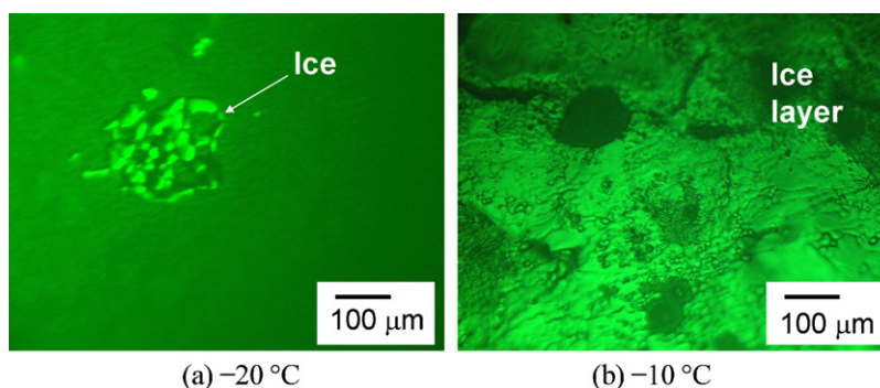
Fig. 8. Micrographs of the cathode catalyst layer surface after the shutdown at –20 °C and –10 °C.
