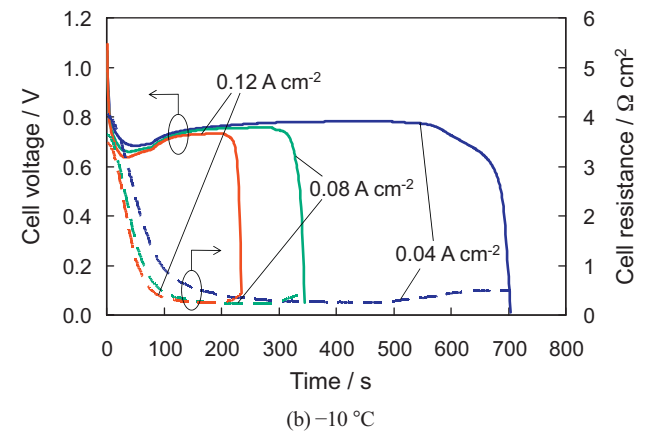
Fig. 7. Cell voltages and resistances for the cold start operation of various current densities at -20^{\circ}\text{C} and -10^{\circ}\text{C} .
