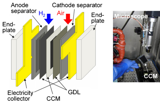
Fig. 1. Experimental apparatus and photo of the inside of the thermostatic chamber.
