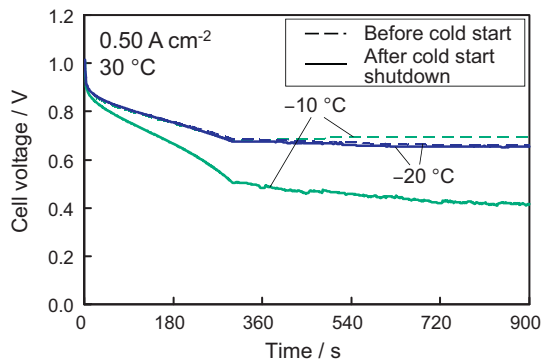
Fig. 10. Plot of the cell performance at 30 °C before and after the occurrence of shutdown due to the cold start at -20 °C and -10 °C.
