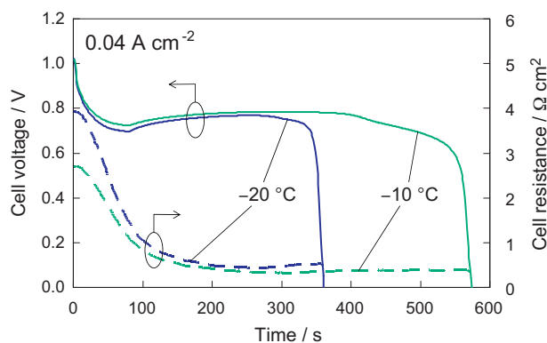
Fig. 4. Cell voltages and resistances for the 0.04 A cm -2 cold start operation at –20 °C and –10 °C.
