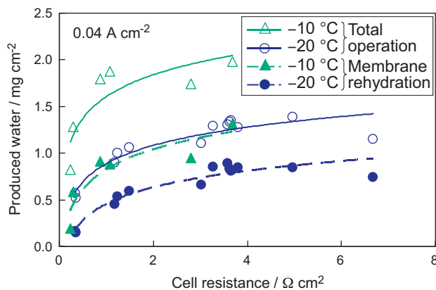
Fig. 5. Amount of water produced in the total operation and in the membrane rehydration at –20 °C and –10 °C; the abscissa is the cell resistance before the cold start.
