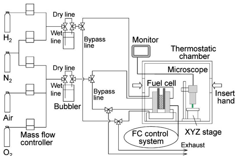
Fig. 2. Schematic outline of the developed arrangement for evaluating the cold start performance and the ice formation inside the cell.
