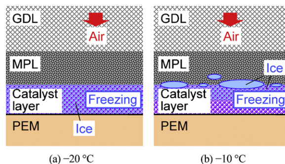
Fig. 9. Experimentally suggested images of the cross-sectional distribution of ice at the shutdown after the cold start at –20 °C and –10 °C.
