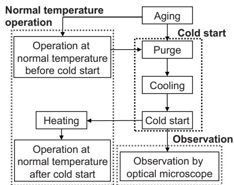
Fig. 3. Experimental procedures of the cold start, the direct observation, and the normal temperature operation.
