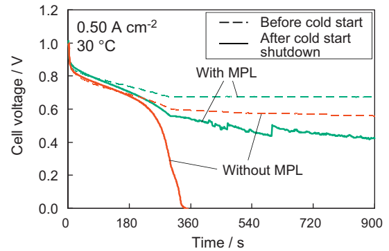
Fig. 11. Plot of the cell performance at 30 °C before and after the occurrence of shutdown due to the cold start with and without the MPL.
