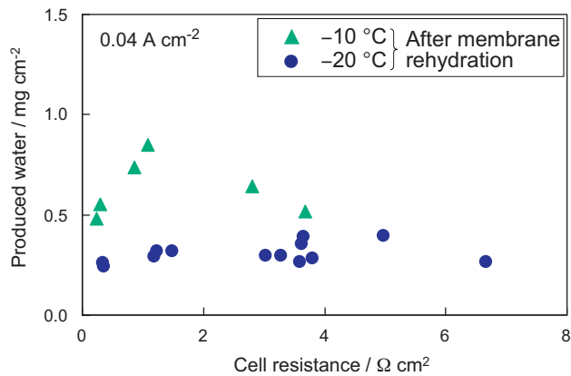
Fig. 6. Amount of water produced during the period from the end of the membrane rehydration till the time of the stop of the operation at -20^{\circ}\text{C} and -10^{\circ}\text{C} .
