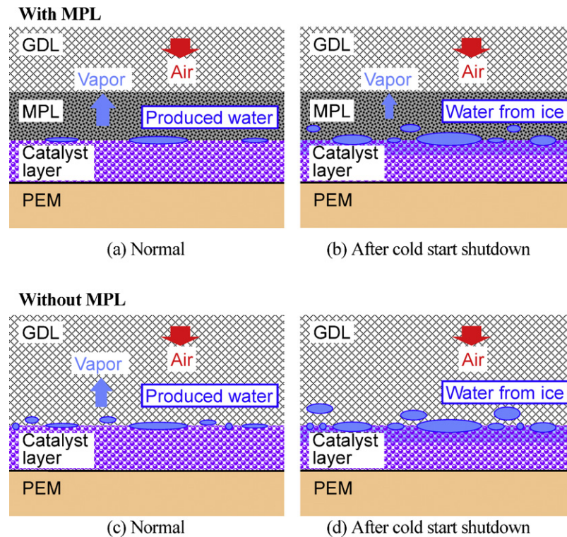
Fig. 13. Experimentally suggested images of the cross-sectional distribution of liquid water at normal operation and after the cold start shutdown operation.
